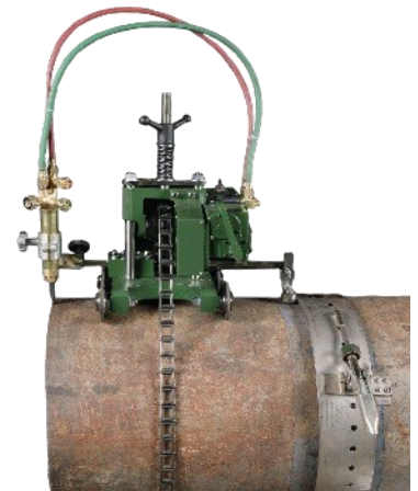
Optional guide rail provides high cutting accuracy, particularly suitable for large pipes. Each guide rail is provided with additional chain links for each maximum pipe diameter.
